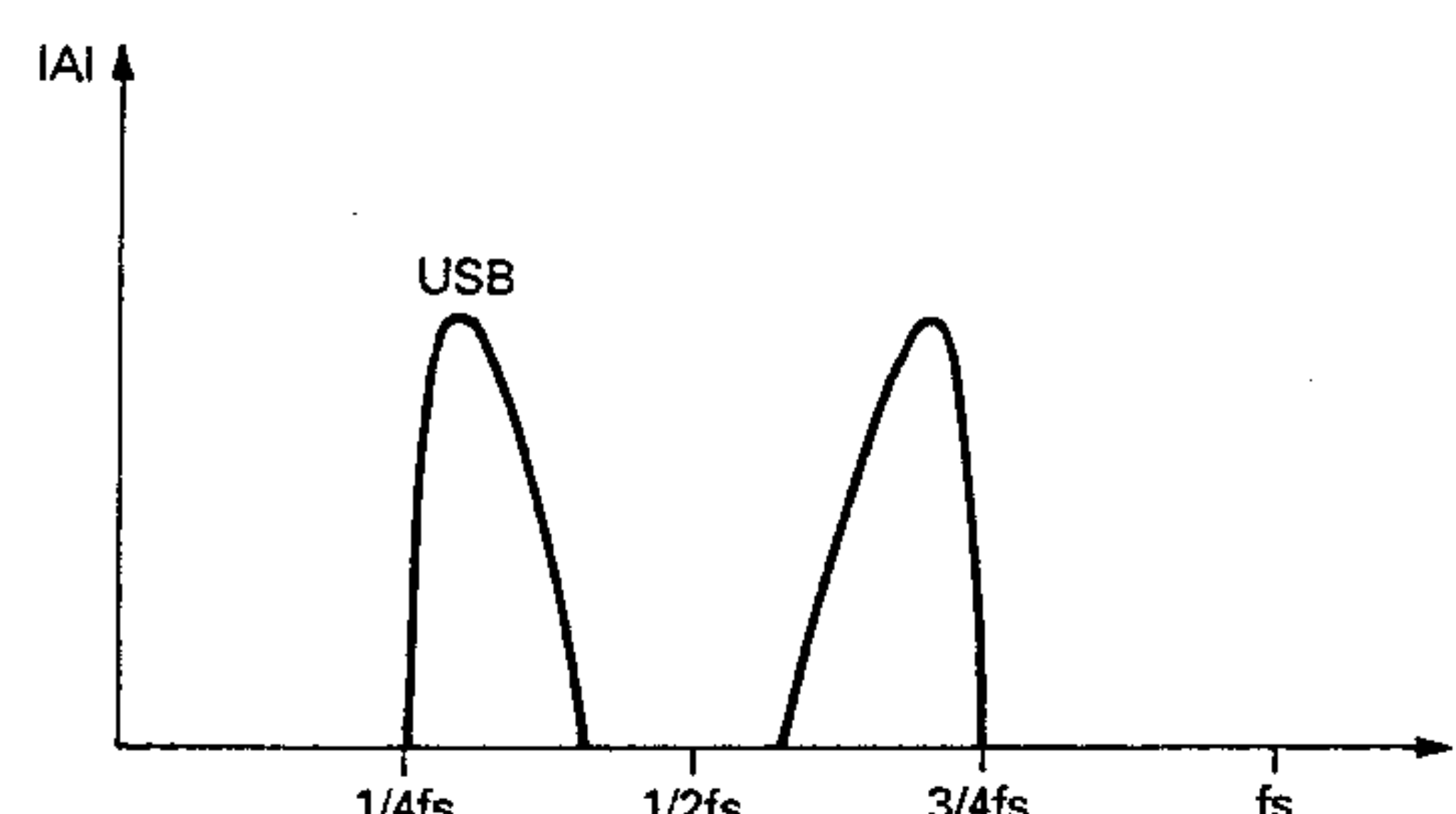
(b) S/H amplifier output spectrum
