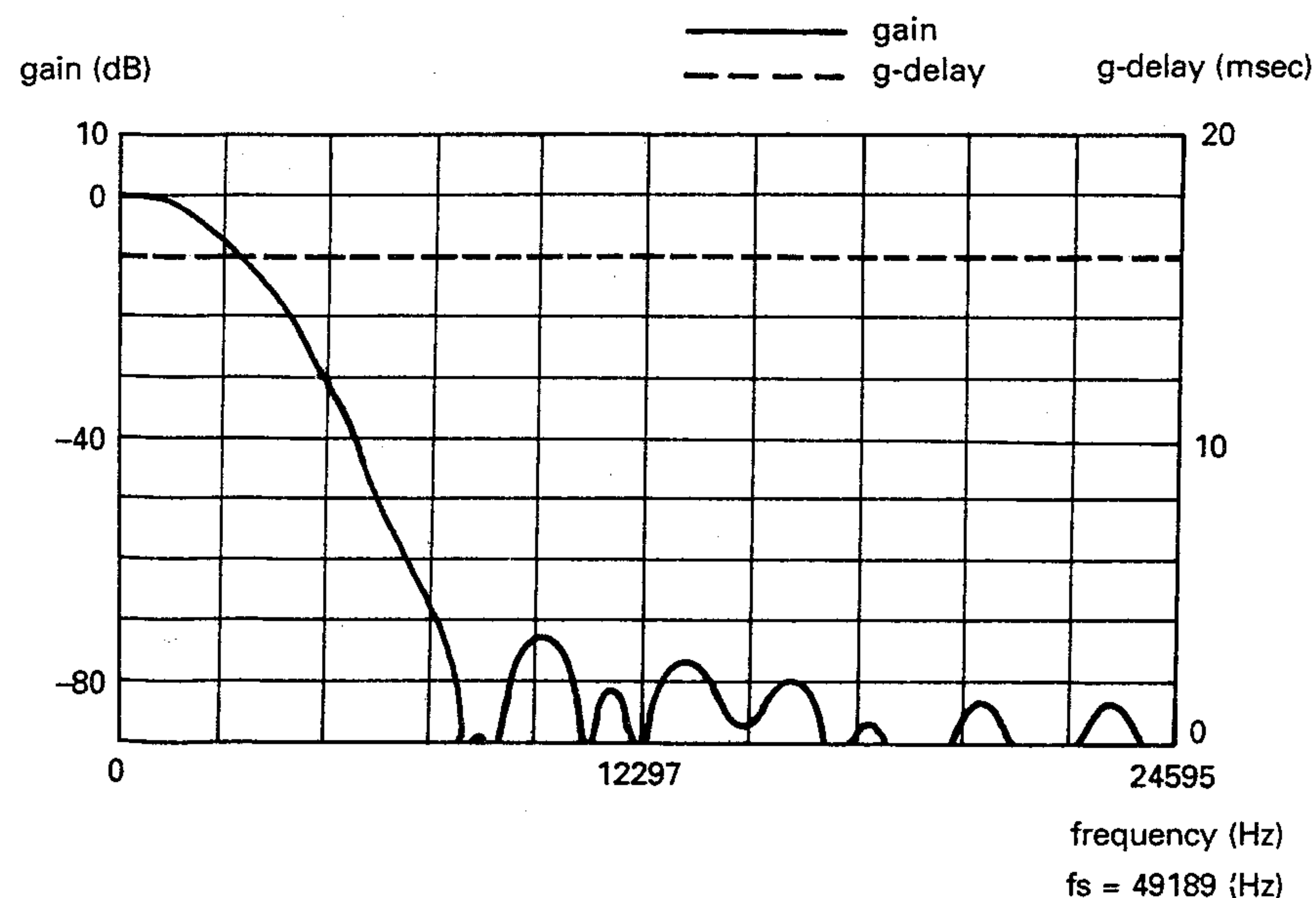
Fig. 10-b FIR filter for FSK frequency characteristics
