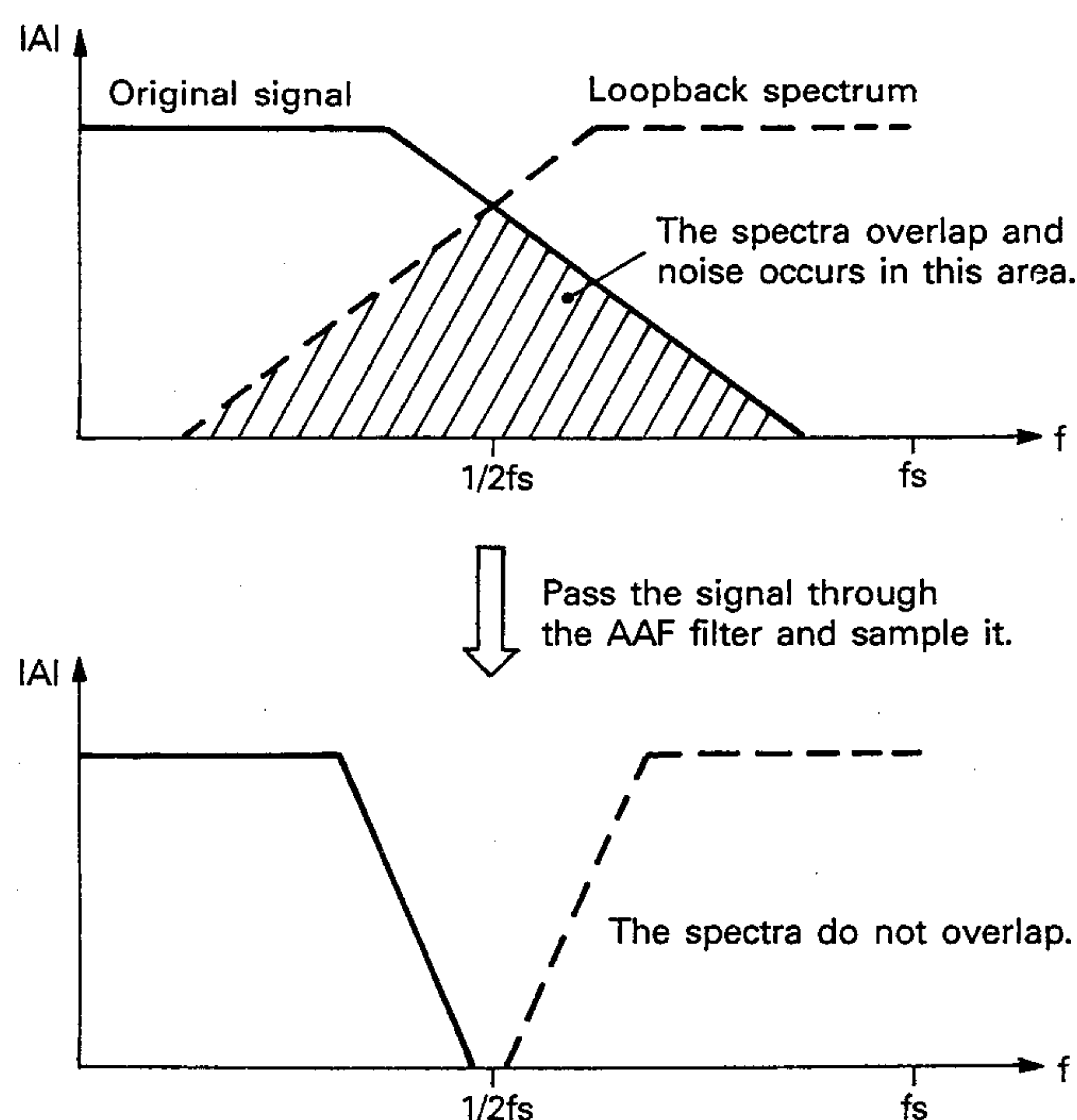
Fig. 4 Loopback distortion
