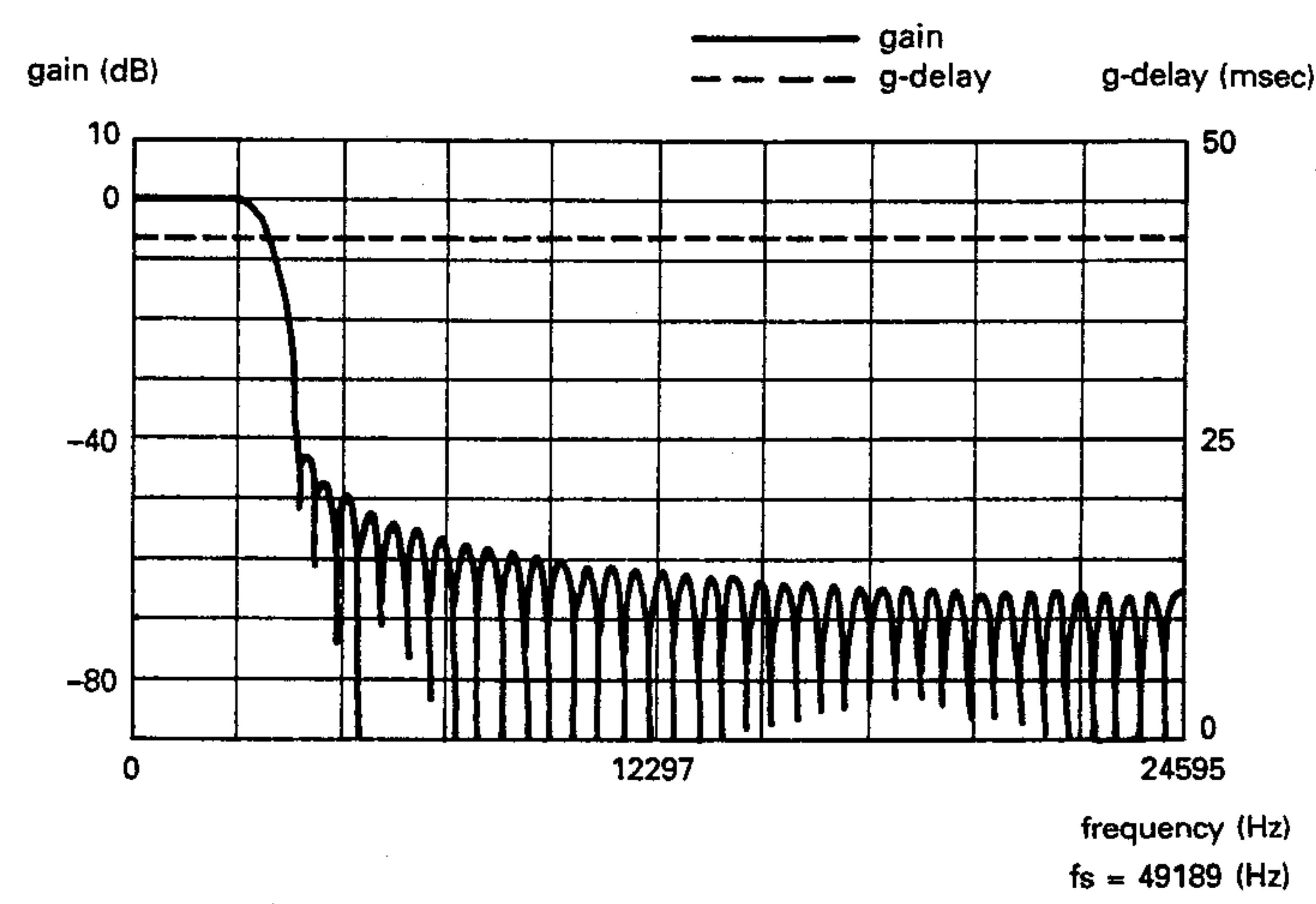
FIR of degree 84
